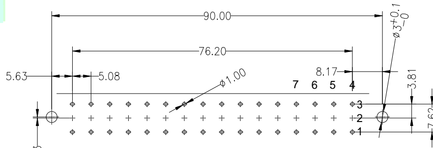
PCB LAYOUT(RECOMMENDED) (TOP VIEW TOL. ±0.05)
